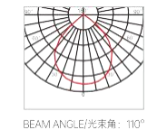
LIGHT DISTRIBUTION CURVE 配光曲线
