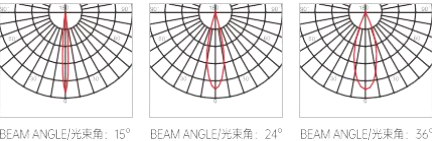
LIGHT DISTRIBUTION CURVE 配光曲线
