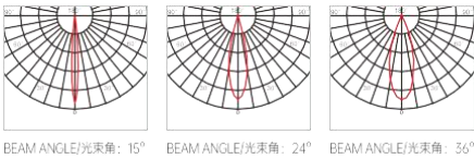
LIGHT DISTRIBUTION CURVE 配光曲线
